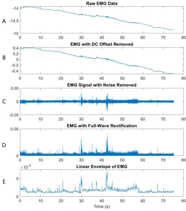
Figure 5: Four steps of EMG signal pre-processing: removing DC offset, denoise, full-wave rectification, and linear envelope.
